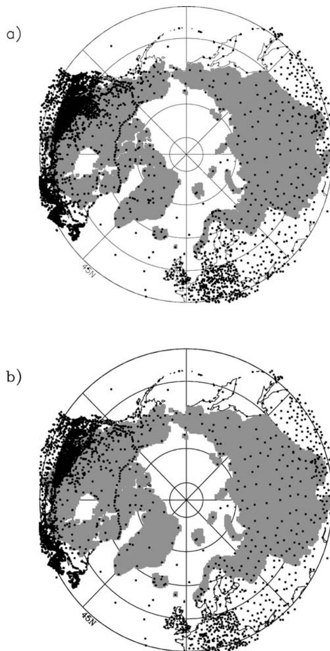
FIGURE 1. Locations of the monthly air-temperature station records for all Arctic stations (a) and for those Arctic stations with data from the period 1961–1990 (b). The light grey shading delineates the Pan-Arctic drainage basin. The map projection is Lambert's Azimuthal Equal Area.
