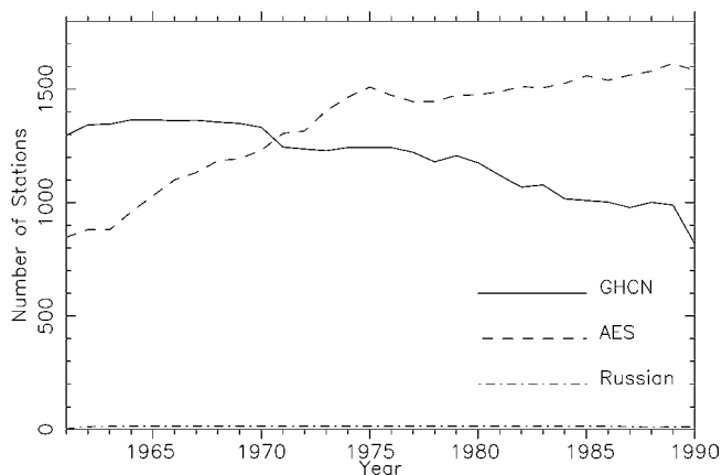
FIGURE 5. Number of stations used in 1961–1990 winter air temperature interpolations, from GHCN v2, AES Canada, and Russian data sets.
