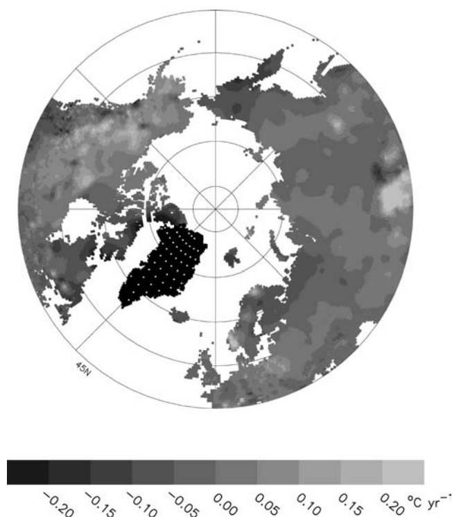
FIGURE 6. Winter average air-temperature trends based on traditionally interpolated yearly winter air-temperature fields.
