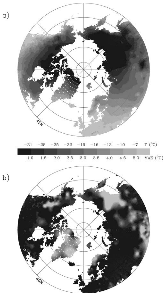
FIGURE 2. Traditionally interpolated winter average air temperature (a) and associated cross-validation MAE (b). The stippling over Greenland indicates that its grid-point values may be questionable and they are not used in computing terrestrial Arctic averages.
