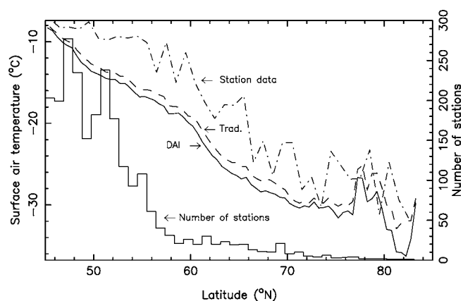
FIGURE 4. Latitudinally averaged winter average air temperature associated with the station records, traditional interpolation, and DAI. Latitude bands are at 0.5^{\circ} increments for the gridded fields and 1^{\circ} increments for the station data (Greenland is not included). The right-hand axis scales the number of stations within the 1^{\circ} of latitude bands, beginning at 45^{\circ}\text{N} .
