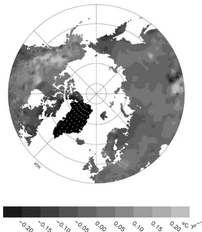
FIGURE 7. Winter average air-temperature trends based on yearly DAI fields.
