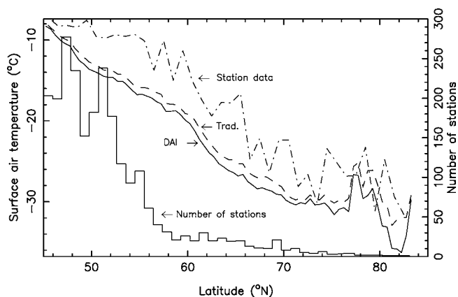
FIGURE 4. Latitudinally averaged winter average air temperature associated with the station records, traditional interpolation, and DAI. Latitude bands are at 0.5 increments for the gridded fields and 1 increments for the station data (Greenland is not included). The right-hand axis scales the number of stations within the 1 of latitude bands, beginning at 45^{\circ}\text{N} .
