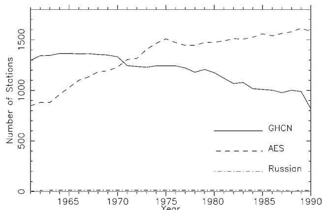
FIGURE 5. Number of stations used in 1961–1990 winter air temperature interpolations, from GHCV v2, AES Canada, and Russian data sets.
